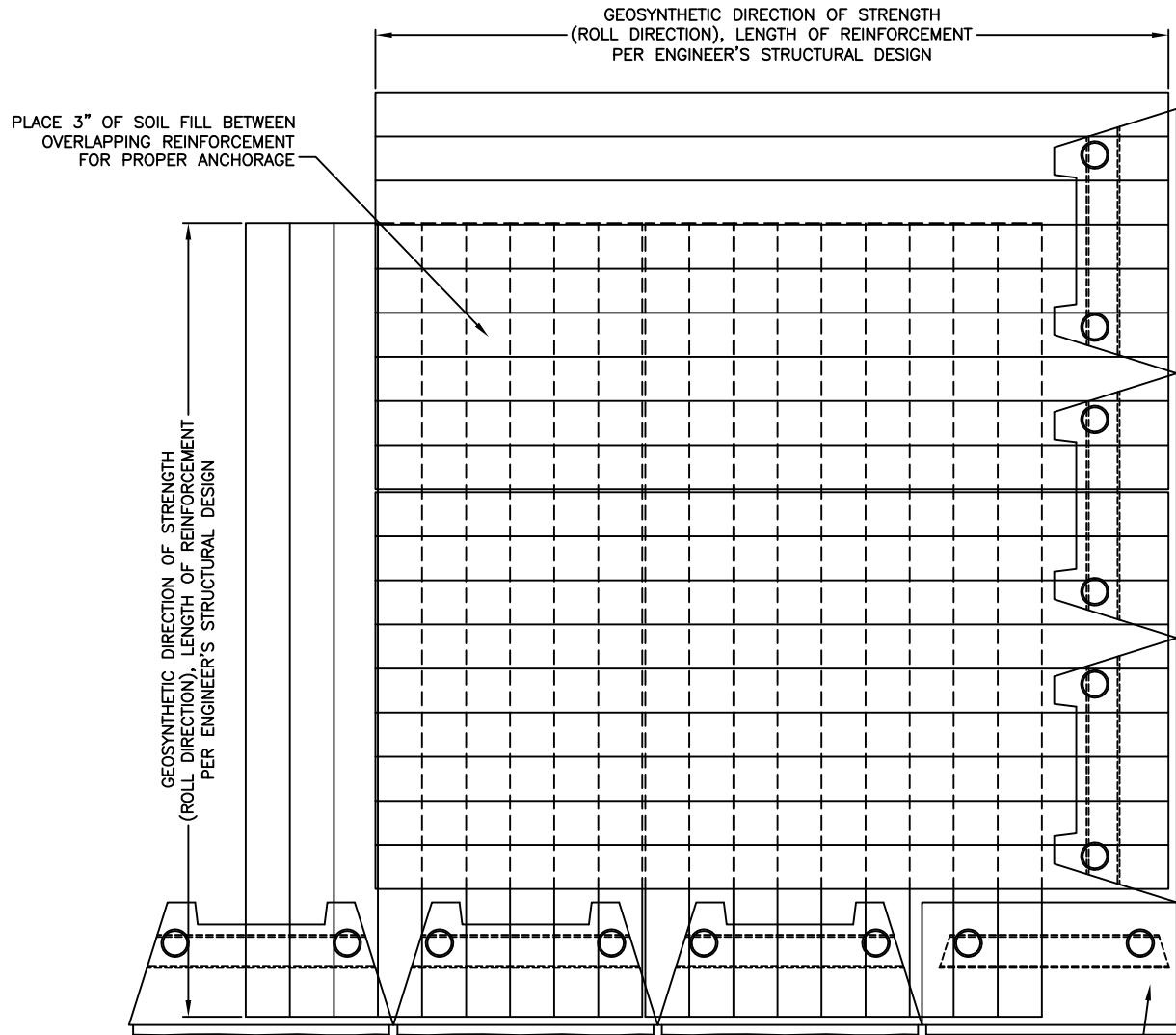
OUTSIDE 90° CORNER 24 INCH UNITS WITH REINFORCEMENT SCALE: NONE
